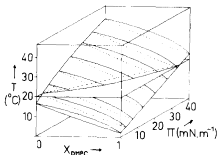
Fig. 2. The phase diagram for a mixture of DMPC and DPPC. The intersections of several isobaric planes with the fluidus surface (—) and solidus surfaces (---) are shown. The plane T = 20^\circ\text{C} is also drawn to show the 'cigar'-shaped figure in the \Pi - x phase diagram. If a system is specified by a point X', \Pi', T' which lies above the fluidus surface, it is an homogeneous fluid, if X', \Pi', T' lies below the solidus surface, it is an homogeneous solid. If it lies between the two it separates into fluid and solid phases whose compositions are specified by the intersection with, respectively, the fluidus and solidus surfaces of a line through X', \Pi', T' parallel to the x -axis. Ideal mixing is assumed and the data are from Ref. 17.
