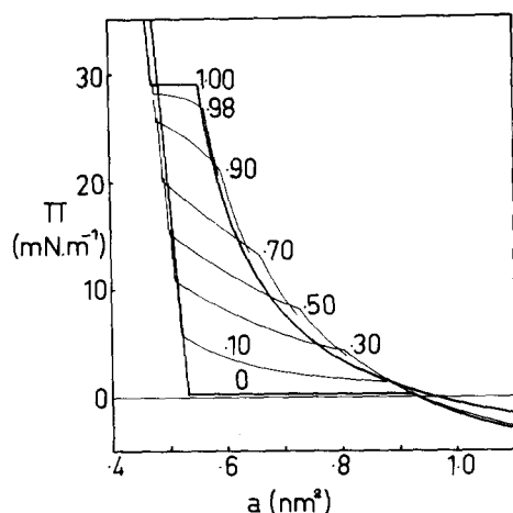
Fig. 4. Calculated \Pi - a isotherms at 16^{\circ}\text{C} for monolayer mixtures of DMPC and DPPC at the air-water interface. The fraction of DMPC is indicated for each curve. The data from Ref. 17 have been used assuming a van der Waals equation of state for the fluid and a small constant compressibility for the solid.
